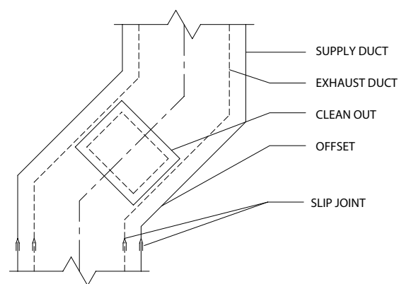
OFFSET
