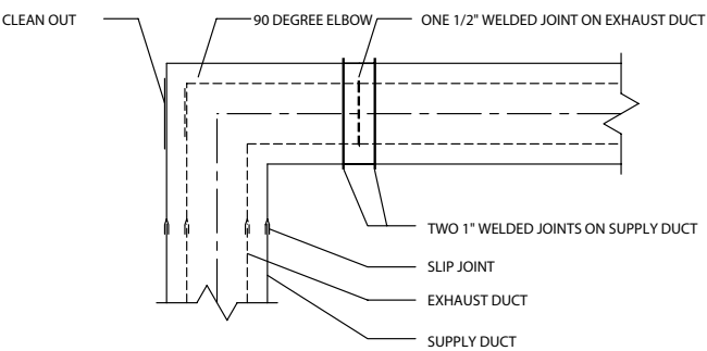
HORIZONTAL DUCT W/WELDED JOINT CONNECTION
