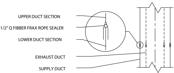
VERTICAL DUCT W/SLIP JOINT CONNECTION
