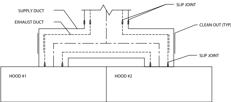
TEE-DUCT
